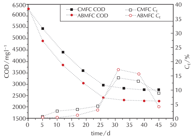
Fig. 4 – Variation of COD and Coulombic efficiency
