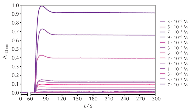
Fig. 3 – Kinetic curves for the proposed redox reaction measured at optimum experimental conditions
