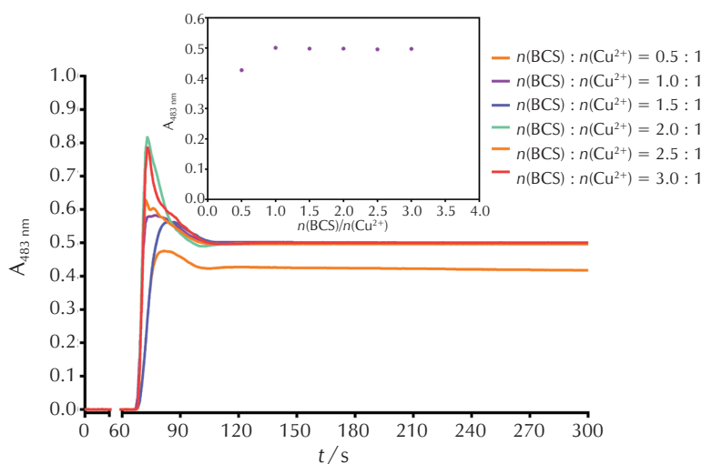
Fig. 2 – Absorbance change as a function of time for kinetic spectrophotometric determination of NAC at different reagent molar ratios. Inset: Dependence of absorbance on reagent molar ratio.
