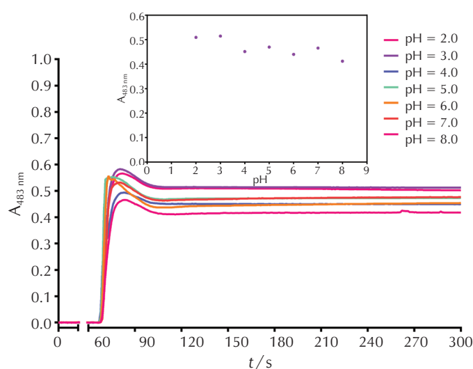
Fig. 1 – Absorbance change as a function of time for the kinetic spectrophotometric determination of NAC at different pH values. Inset: Dependence of absorbance on pH.
