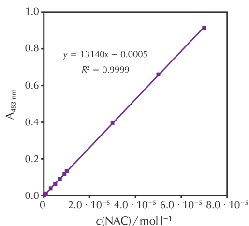
Fig. 4 – Fixed-time method calibration curve (120 s)
