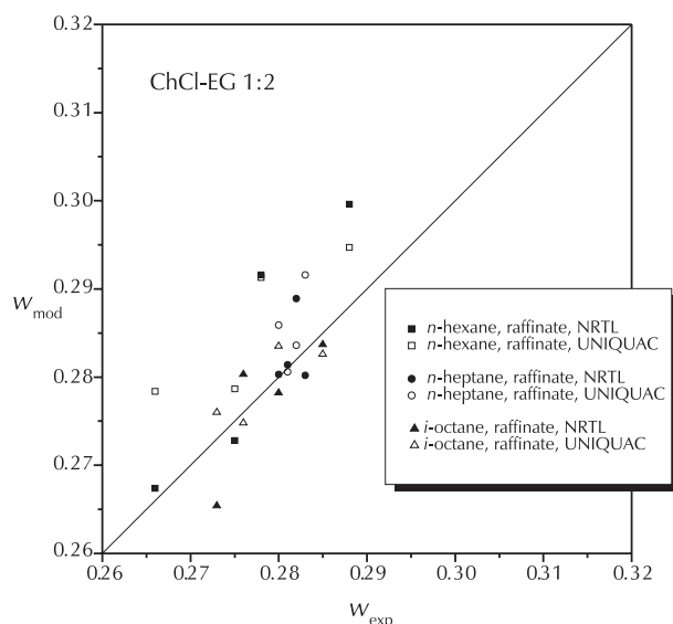
Fig. 11 – Comparison of experimental and calculated component distributions (mass fractions) for quasi-seven-component systems with DES / model gasoline ratio of 0.25 \text{ kg kg}^{-1} – middle mass fraction range
