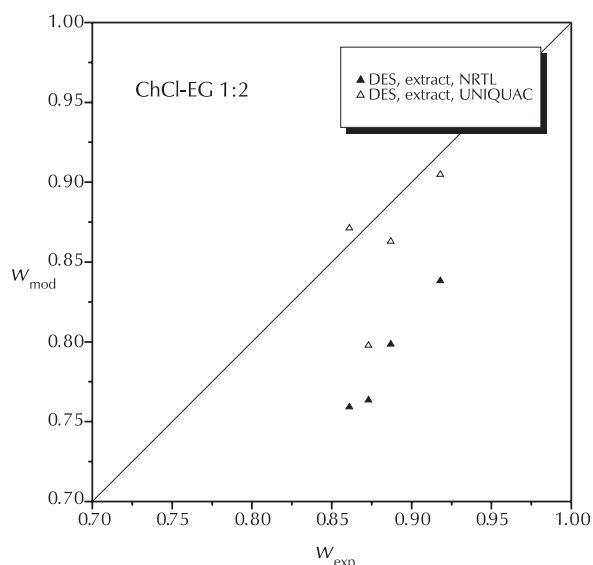
Fig. 12 – Comparison of experimental and calculated component distributions (mass fractions) for quasi-seven-component systems with DES / model gasoline ratio of 0.25 \text{ kg kg}^{-1} – higher mass fraction range
