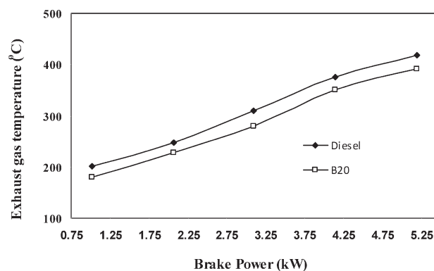
Fig. 8 – Exhaust gas temperature of B20 and diesel with respect to brake power
