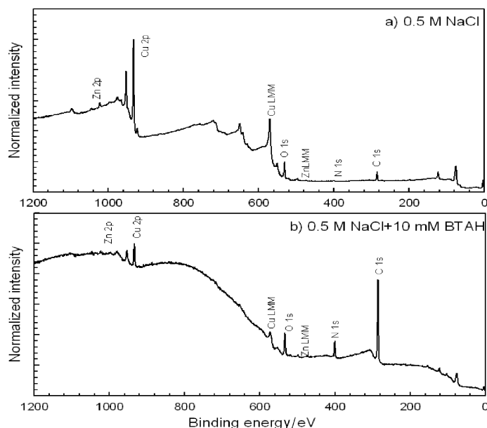
Fig. 4 – XPS survey spectra for films formed on Cu-10Zn alloy in 0.5 M NaCl in the presence and absence of 10 mM BTAH
