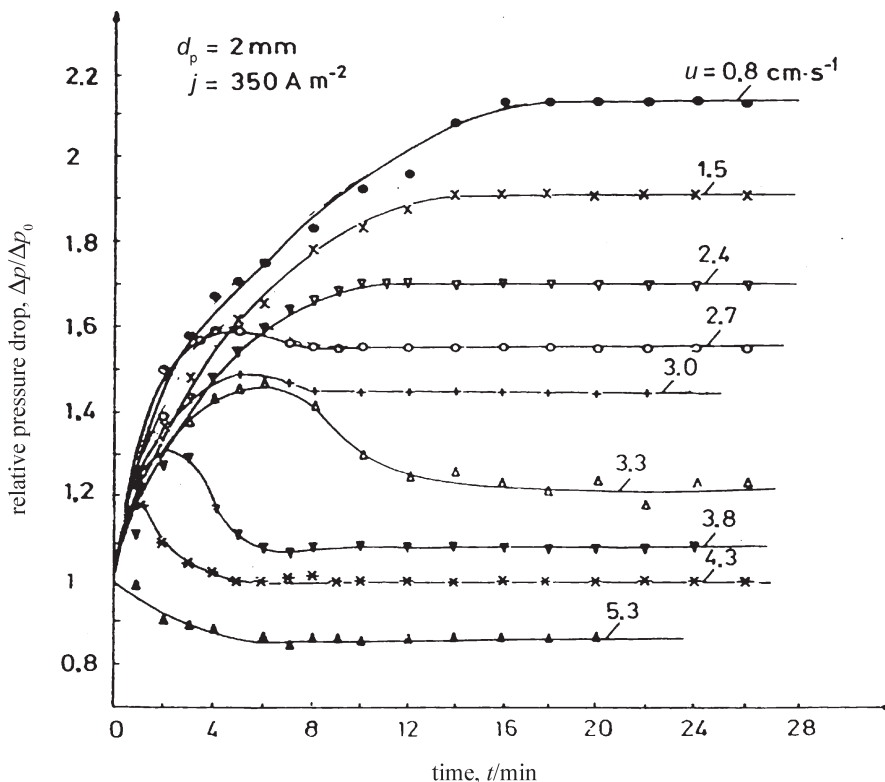
Fig. 7 – Relative pressure-drop behavior with time for different electrolyte velocities 56
