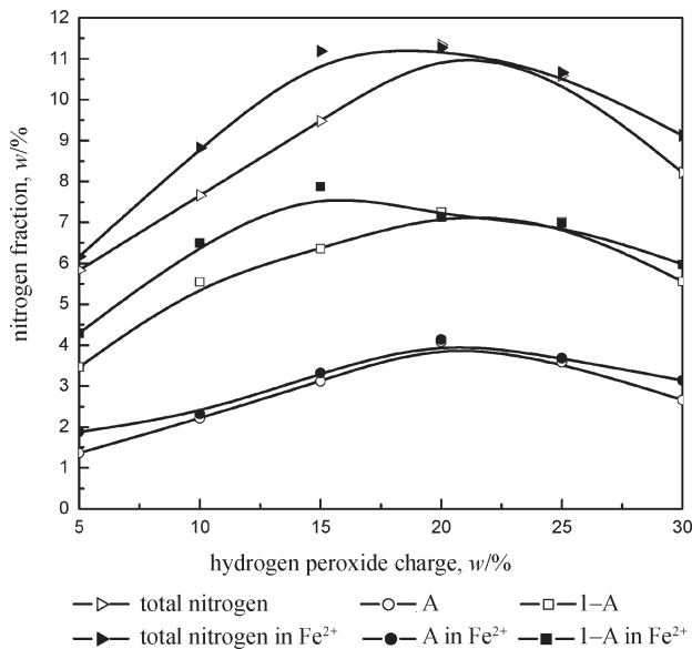
Fig. 5 – Effect of hydroperoxide charge on nitrogen content of lignin with \text{Fe}^{2+} catalysis under reaction temperature 120\text{ }^\circ\text{C} , reaction time 90 min and ammonia charge 20 %
