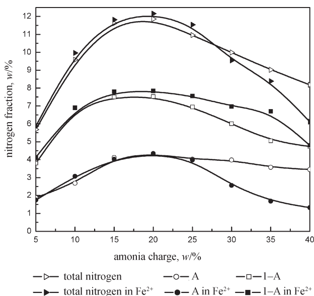
Fig. 6 – Effect of ammonia charge on nitrogen content of lignin with \text{Fe}^{2+} catalysis under reaction temperature 120\text{ }^\circ\text{C} , reaction time 90 min and hydrogen peroxide charge 20 %
