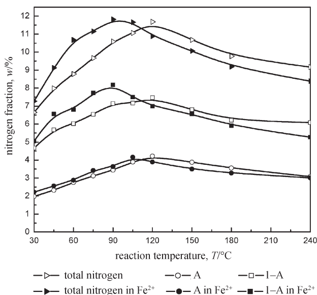
Fig. 3 – Effect of reaction temperature on nitrogen content of lignin with Fe 2+ catalysis under reaction time 90 min, ammonia charge 20 % and hydrogen peroxide charge 20 %
